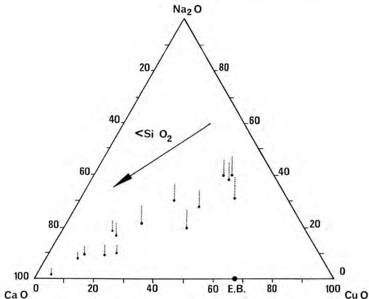
Figure 10.1. Compositional variation of analyses of turquoise material from this study. Length of vertical bars proportional to \text{SiO}_2 content. Full analyses are given in Table 10.5. Composition of Egyptian blue indicated by E.B.
