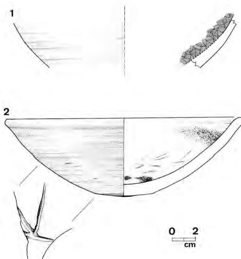
Figure 10.7. 1. Possible reconstruction taken from sherd adhering to purplish frit, from Amarna, Petrie Museum UC 36457. 2. Red slipped bowl from glassworking area, with traces of frit and soot marks on interior, and a small area of frit on the base; the owner's mark (scratched into the surface after firing) on outer body now partly lost, Petrie Museum UC 36460.
